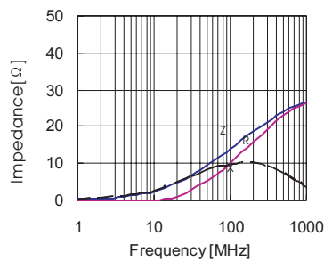
CBM160808U121T
