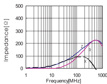
CBM160808U121T
